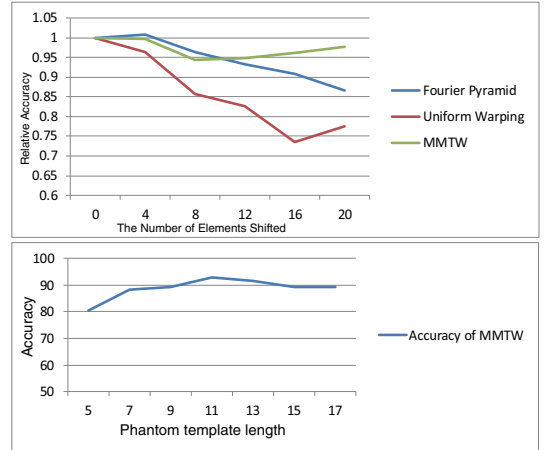
Figure 4. The robustness of the methods to temporal shifts and phantom template length.
